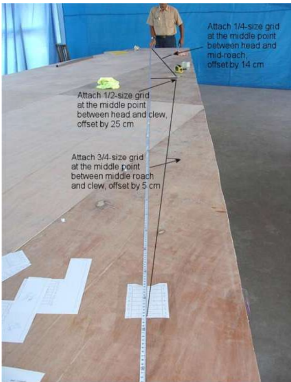
Figure G.2.4.4 Leech point scales
