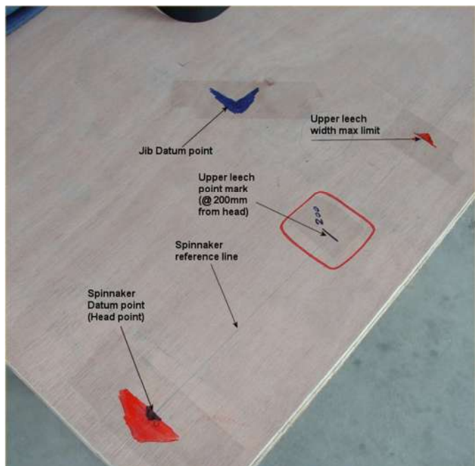
Figure G.2.4.8 Spinnaker measurement marks
