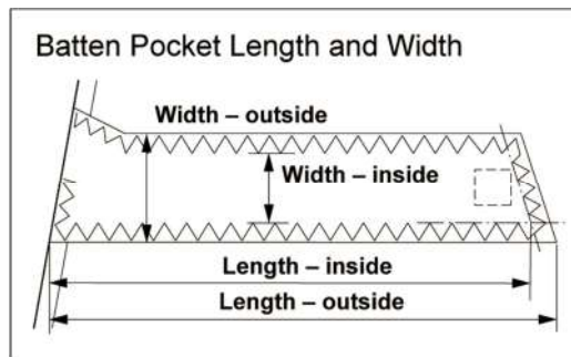
Figure G.4.4 Batten pocket length and width measurement.
