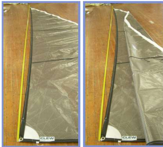
Figures G.2.3.1 & G.2.3.2 Leech flattening before and after flaking.
