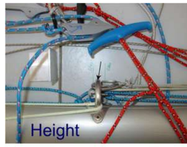
Spinnaker hoist height (left) with the halyard held at 90° to the spar. Spinnaker pole fitting height (right) from the center of the fitting.
