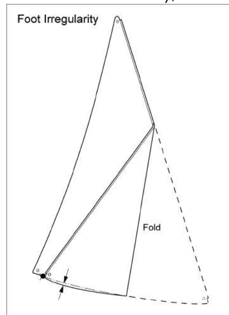
Figure G.4.5 Foot irregularity.
