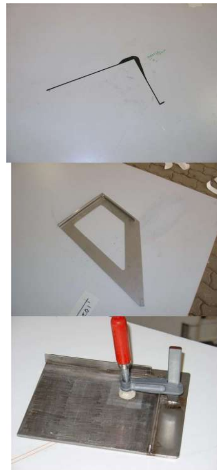
Figure G.2.4.3 Head point jig
