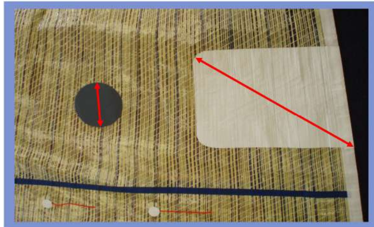
Figure G.4.2 Chafing patch size.
