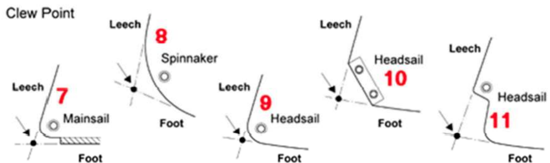
Figure G.2.1.2 Clew point, ERS definition.
