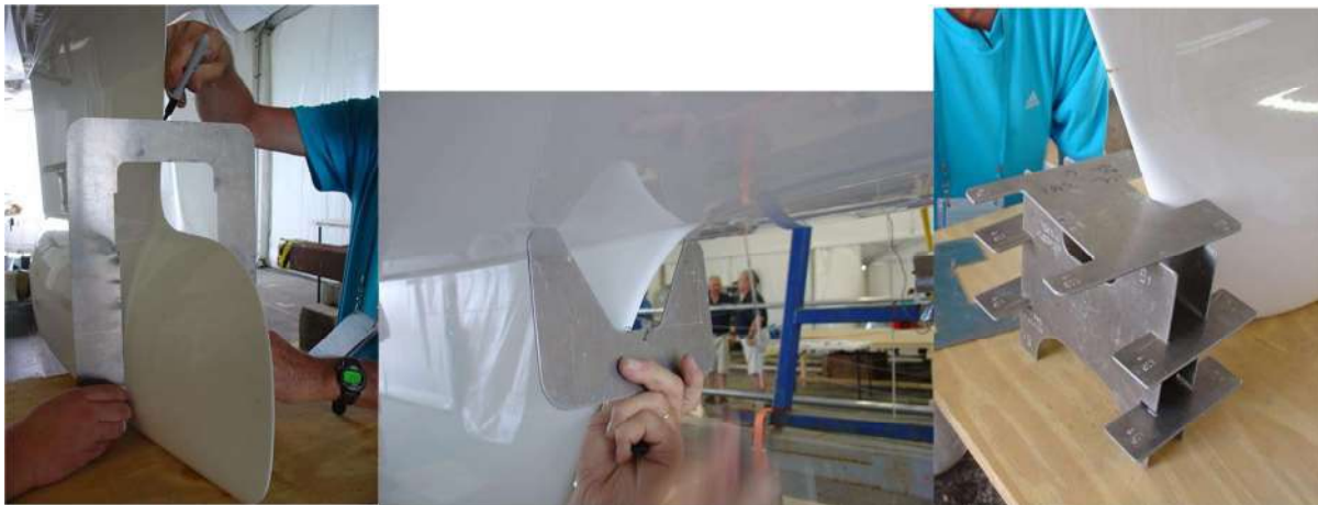
Figure E.2.7 Section marking.
