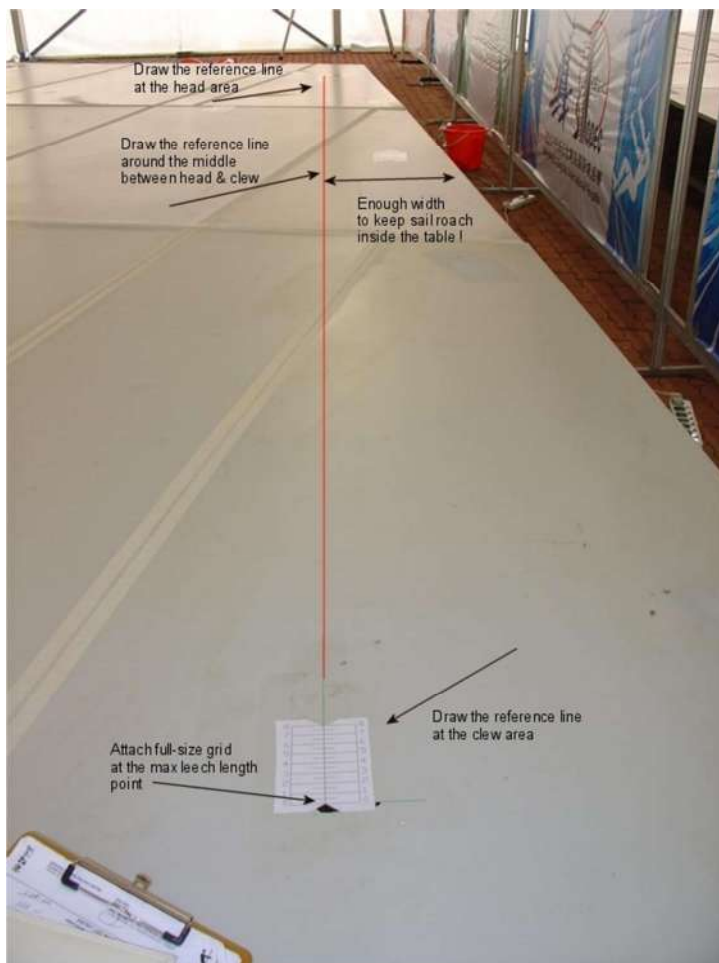
Figure G.2.4.2 Leech length scale
