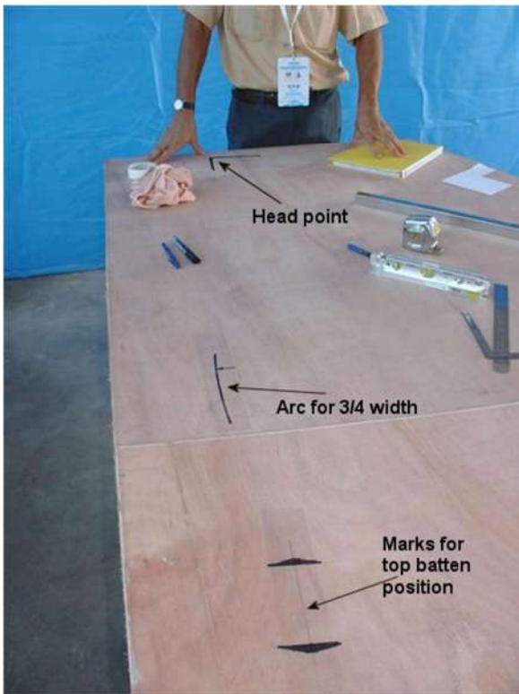
Figure G.2.4.6 Other measurement marks rules
