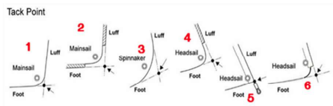
Figure G.2.1.1 Tack point, ERS definition.
