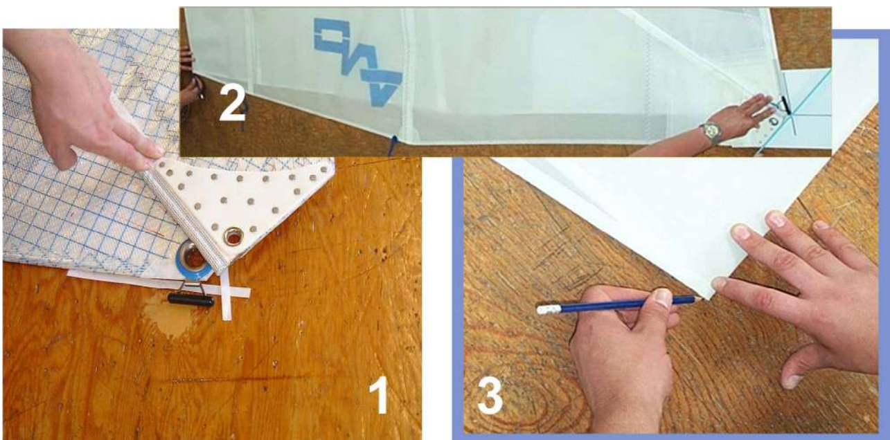
Figure G.2.2.1 Half leech point.
