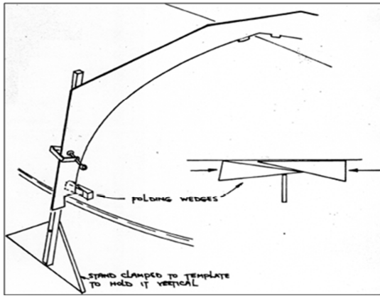
Figure D.1.4.1 Template support
